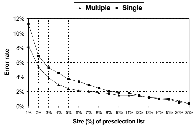
Figure 6: Multiple-SCHMM vs. Single-SCHMM.
