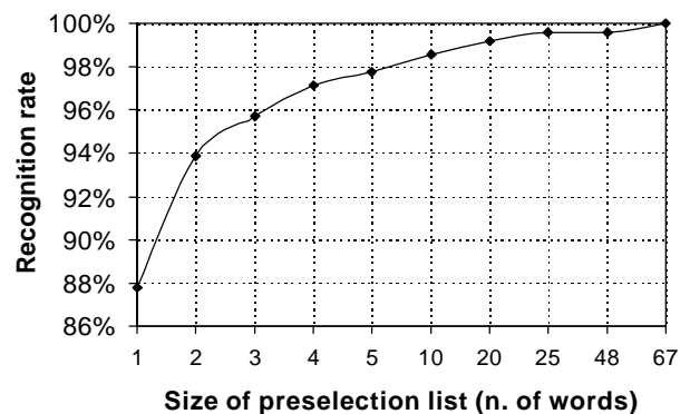
Figure 3: Recognition rate for a clean speech, speaker dependent task with 2000 words dictionary size
