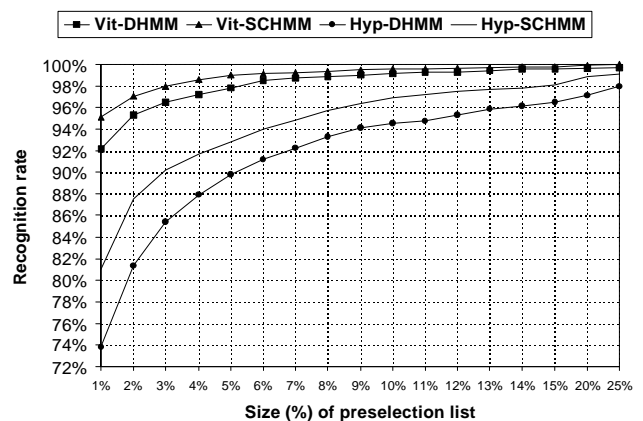
Figure 4: Comparison of Viterbi results for DHMM and SCHMM, along with the equivalent hypothesis subsystems.
