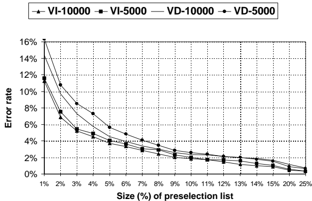
Figure 7: Comparison between VD and VI tasks for 5000 and 10000 words dictionaries. SCHMMs, 25 clustered units.
