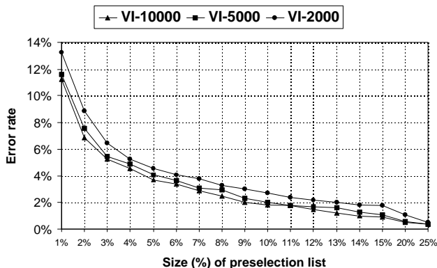
Figure 8: Effect of dictionary size in error rate. SCHMM 25 automatic units, VI data.
