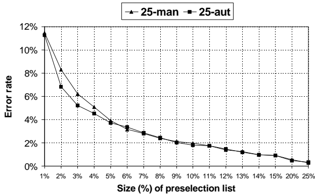
Figure 5: Comparison of manual vs. automatic selection of units.
