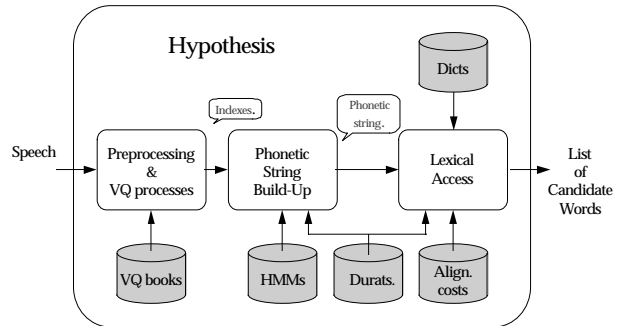
Figure 2: Hypothesis Module Architecture
