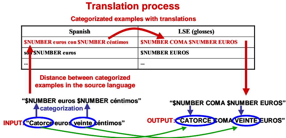
Figure 3. Translation process in an example-based translation system
