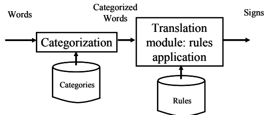
Figure 4. Translation process in a rule-based strategy
